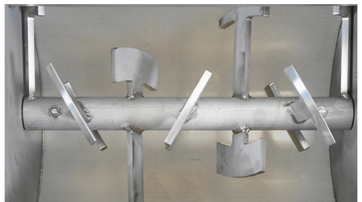
77-PV0077/C Detail of drum with helical mixing shaft
