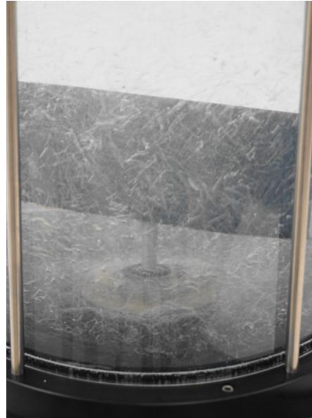
Detail of cavitation system, it allows water to be de-aired much faster than when only using vacuum
