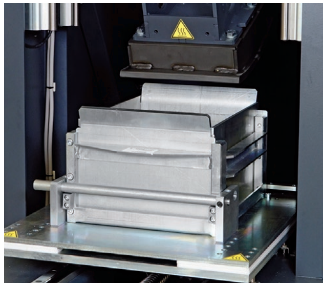
Detail of segment head and mould
