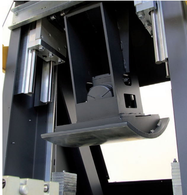
Detail of segment head incorporating vibration unit
